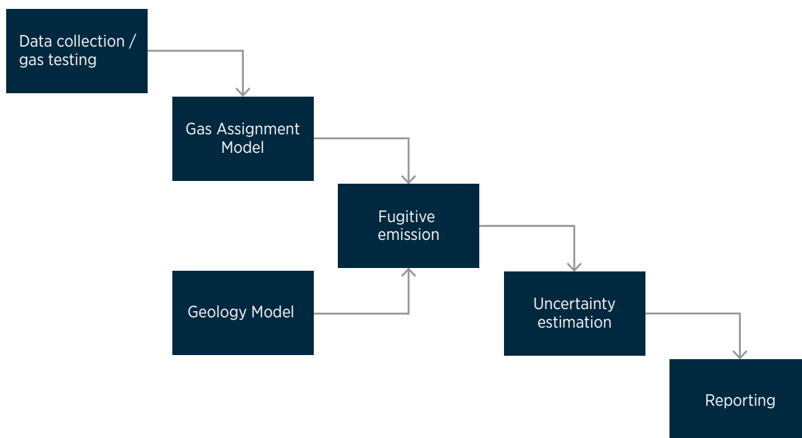
Figure 3.19 Surface mines: emissions estimation process flowchart for companies
