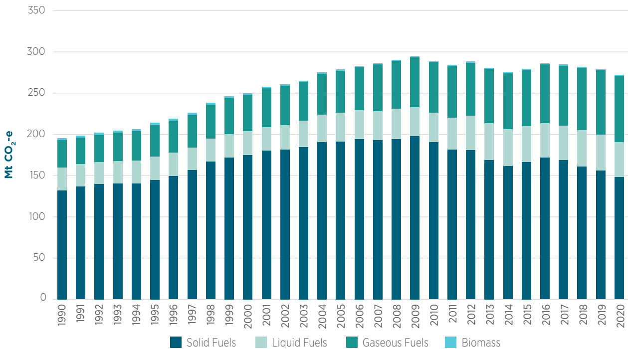
Figure 3.2 Total CO 2 -e emissions from stationary energy combustion by fuel, 1990–2020
