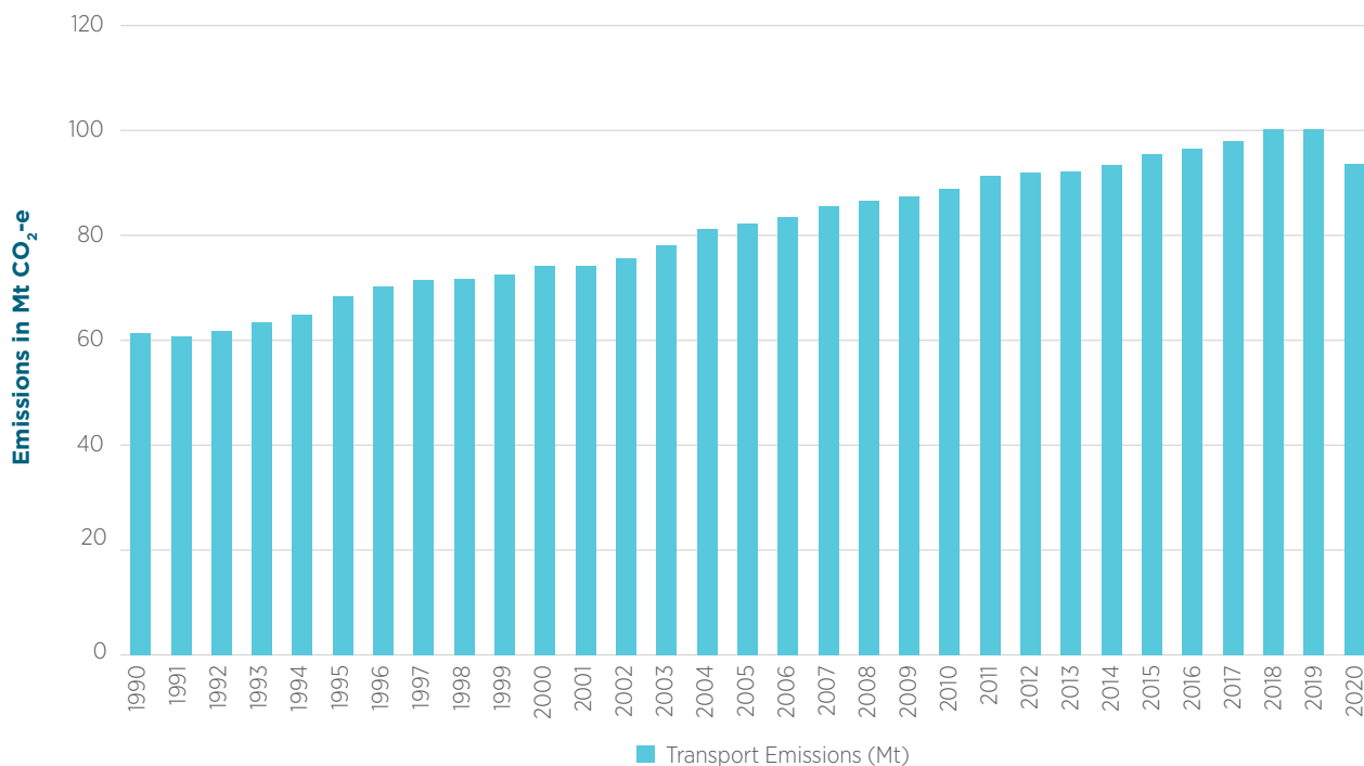
Figure 3.4 Total transport emissions, 1990–2020
