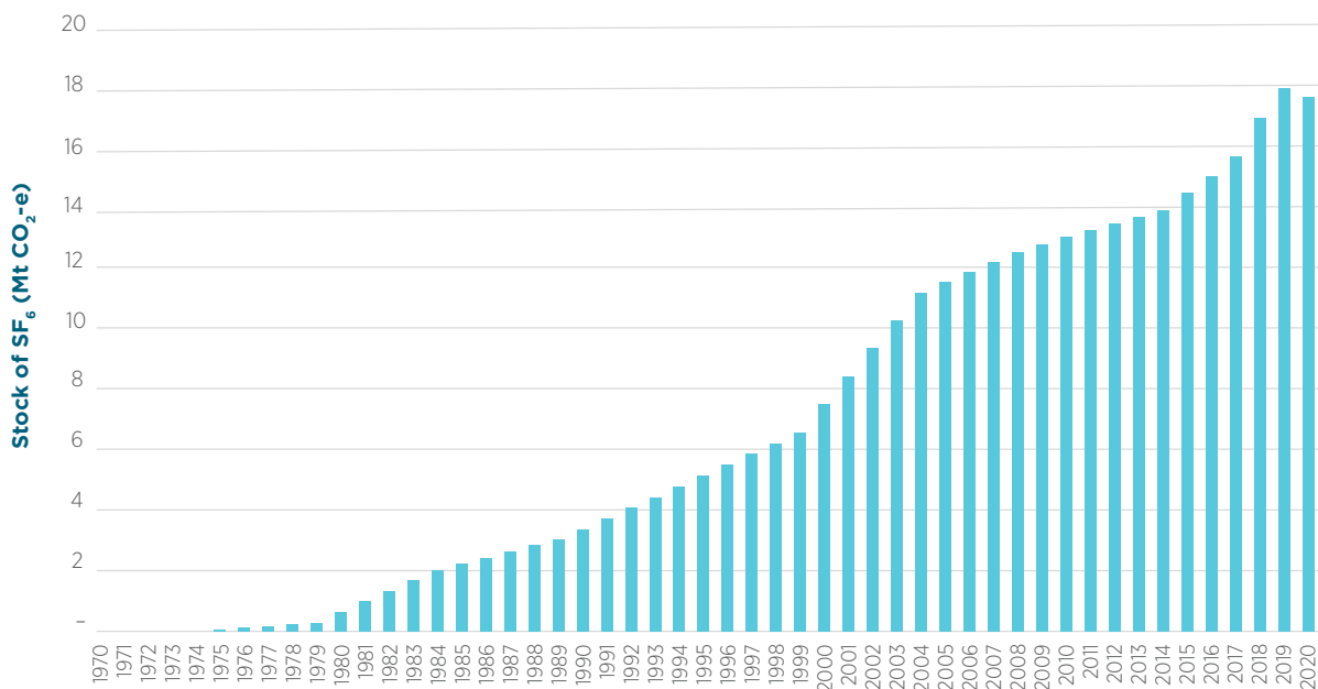
Figure 4.16 Estimated stock of SF 6 in Australia (Mt CO 2 -e)
