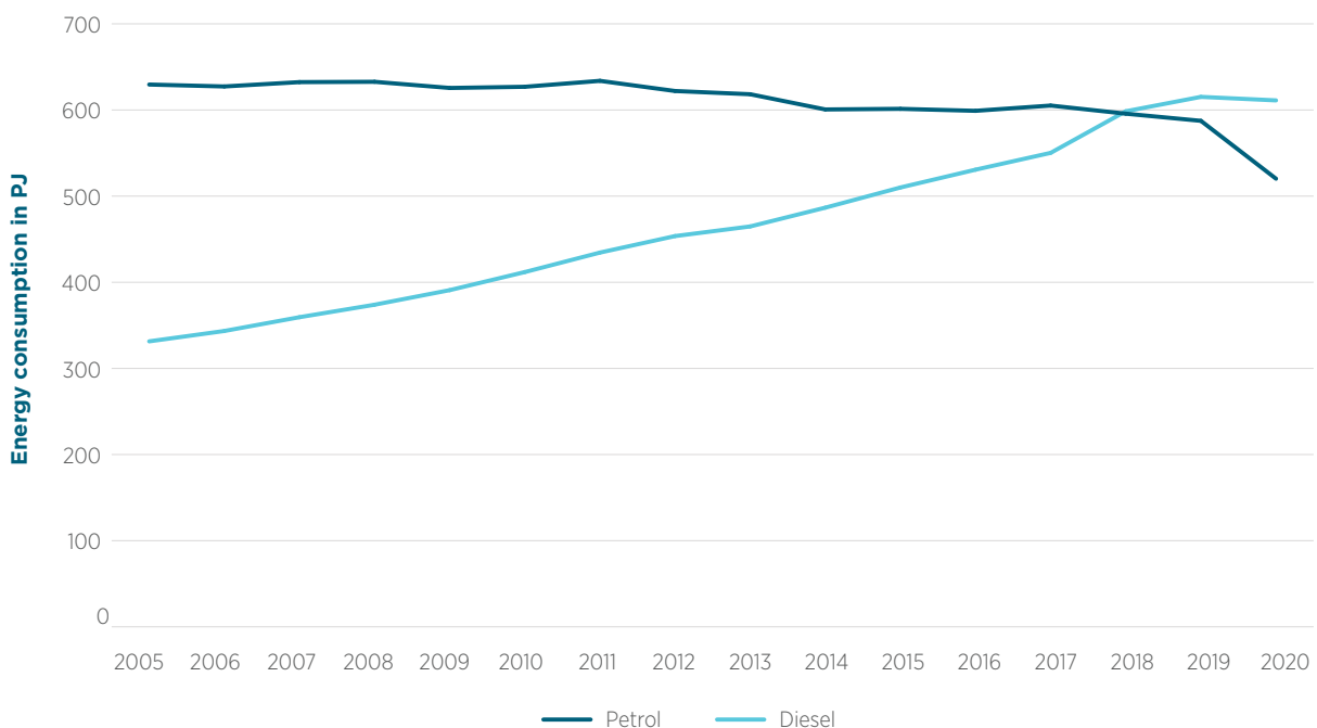
Figure 3.5 Energy consumption in road transport by fuel type (2005–2020)
