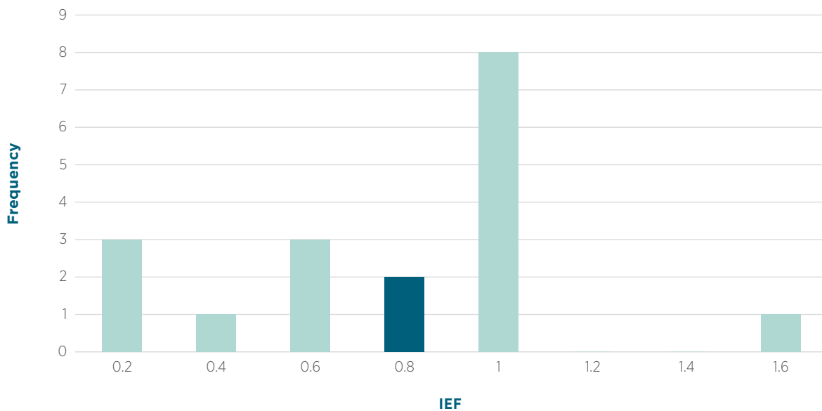
Figure 3.23 Implied emission factor (IEF) for methane from solid fuel surface mines (kg/t) for Annex I countries (2019) and IEF for Australia (2020)
