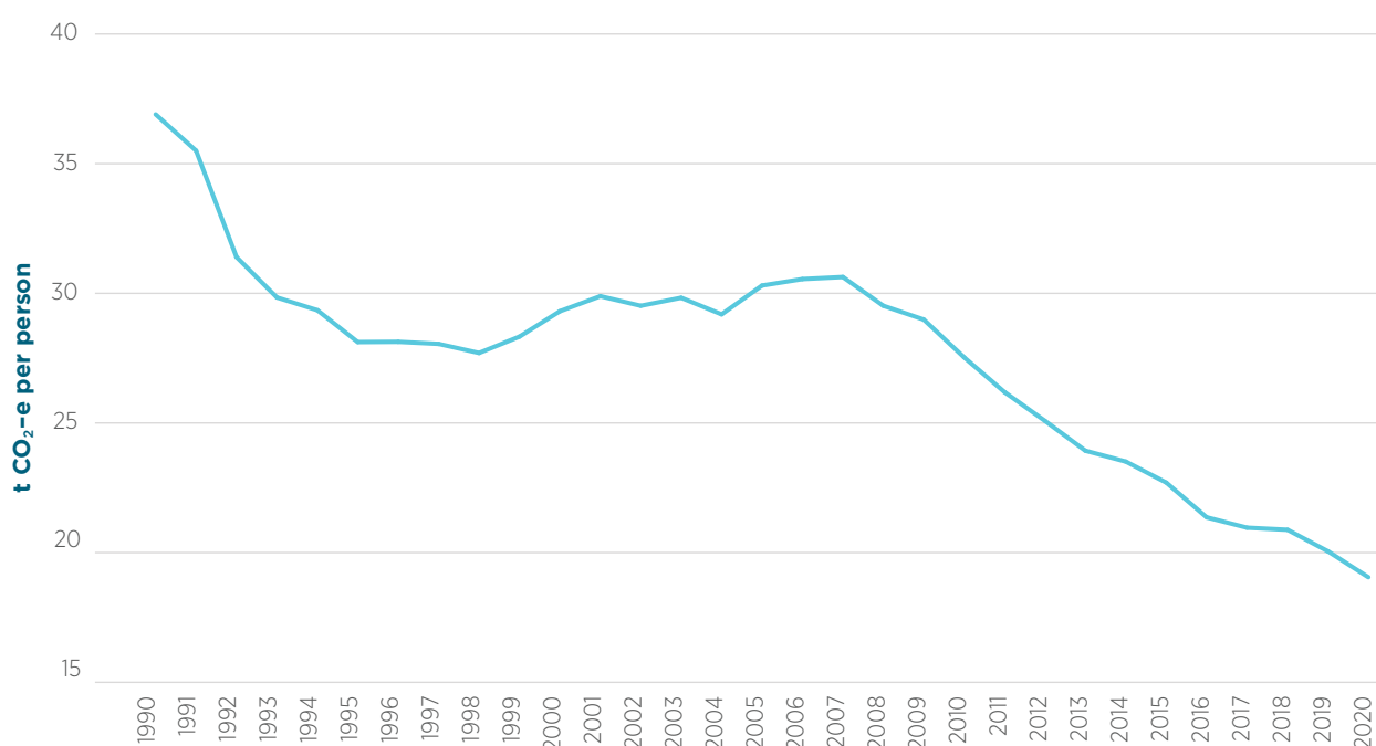
Figure 2.3 Emissions per capita, Australia (t CO 2 -e per person)
