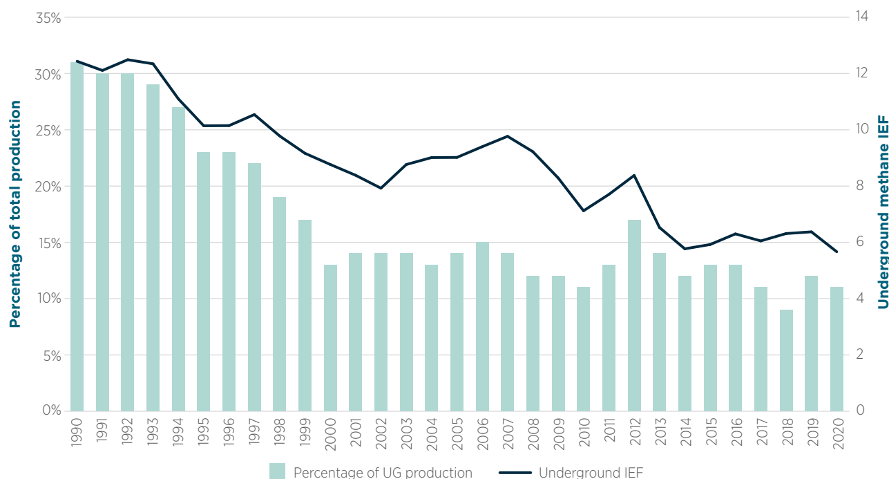
Figure 3.24 Decline of the overall underground coal mine methane implied emission factor compared with the fall in production from the high gas content Southern Coalfield
