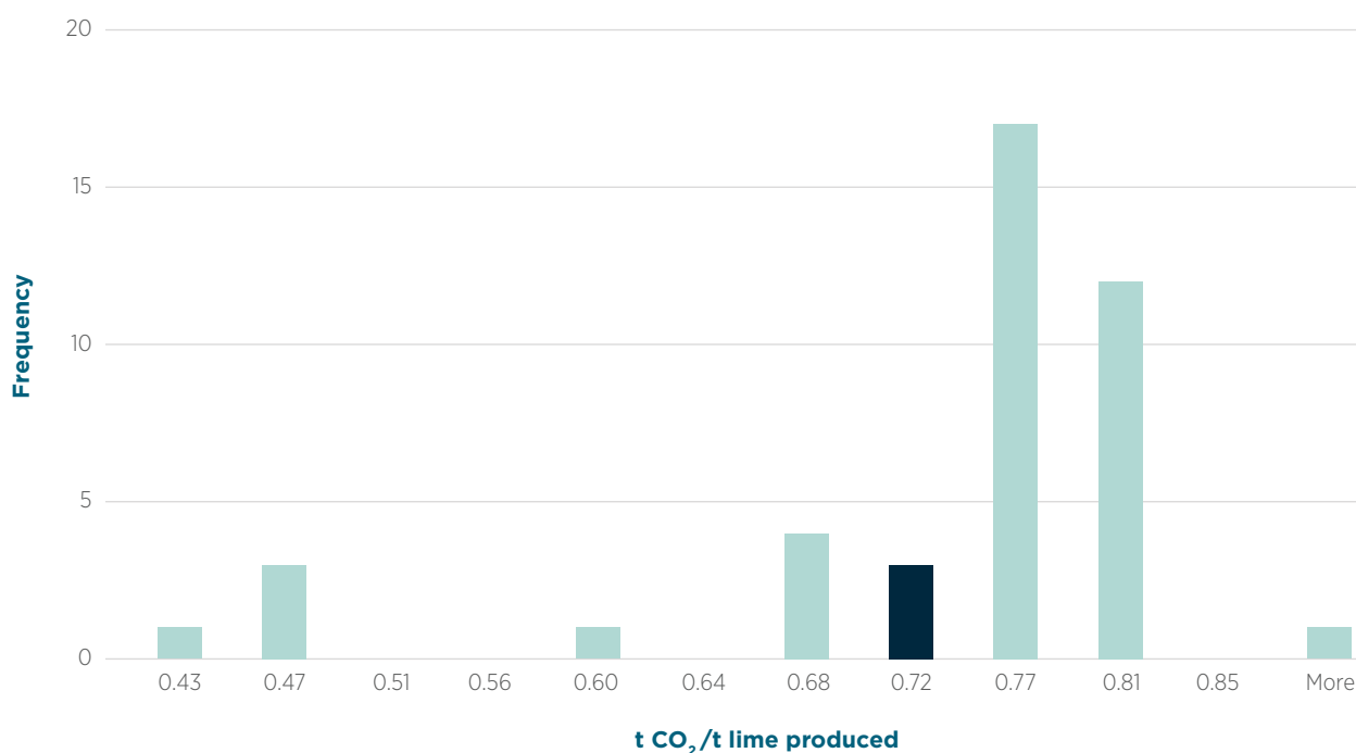
Figure 4.3 Lime production implied emission factors for Annex I countries (2019 Inventory) and Australia (2020 Inventory)
