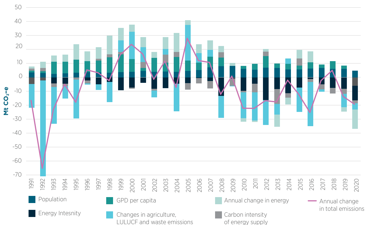
Figure 2.9 Annual change in total emissions from underlying drivers: Australia 1991–2020 (Mt CO 2 -e)
