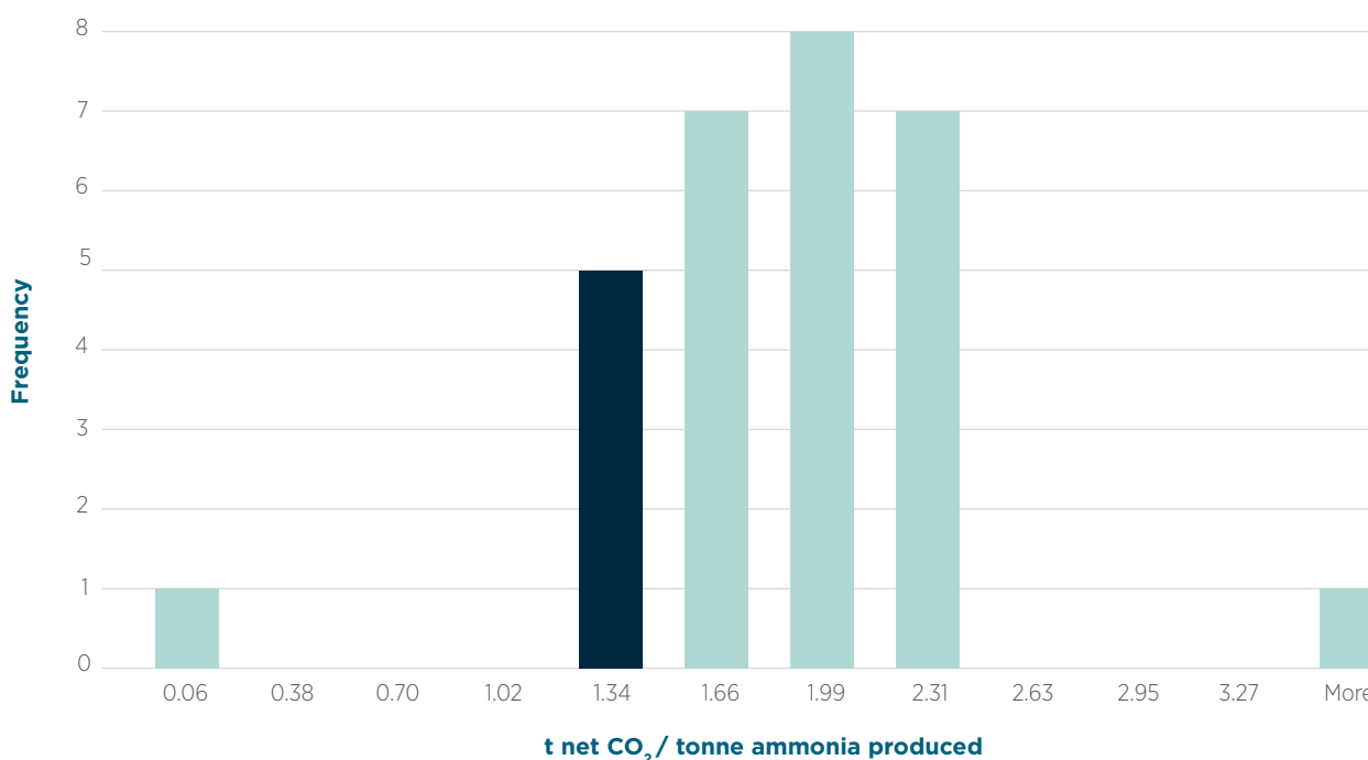
Figure 4.5 Ammonia implied emission factors for Annex I countries (2019 Inventory) and Australia (2020 Inventory)
