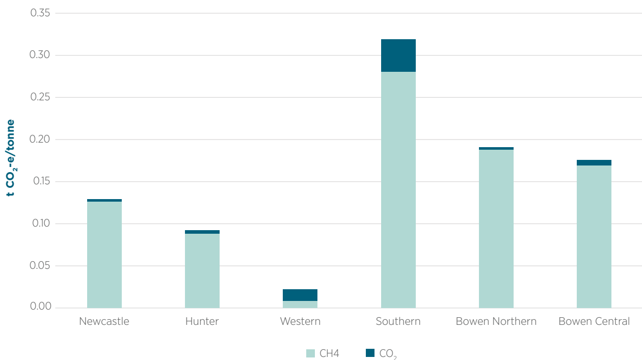
Figure 3.18 The gas content profile of Australian underground production by coal field
