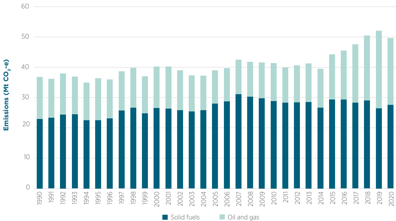
Figure 3.7 CO 2 -e fugitive emissions by category, 1990–2020
