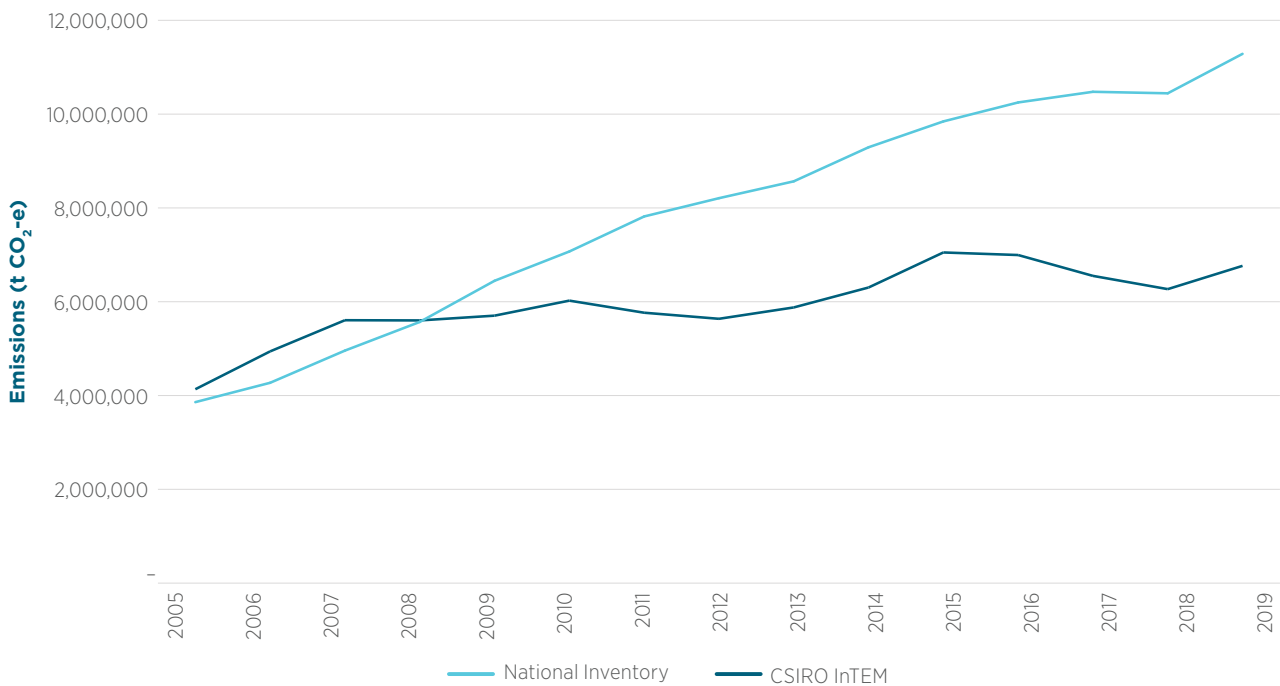
Figure 4.9 Comparison of Inventory HFC emission estimates with estimates derived from Cape Grim measurement data
