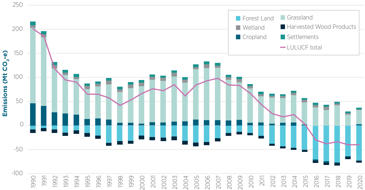
Figure ES.02 Total emissions from LULUCF, Australia, 1990–2020 (Mt CO 2 -e)
