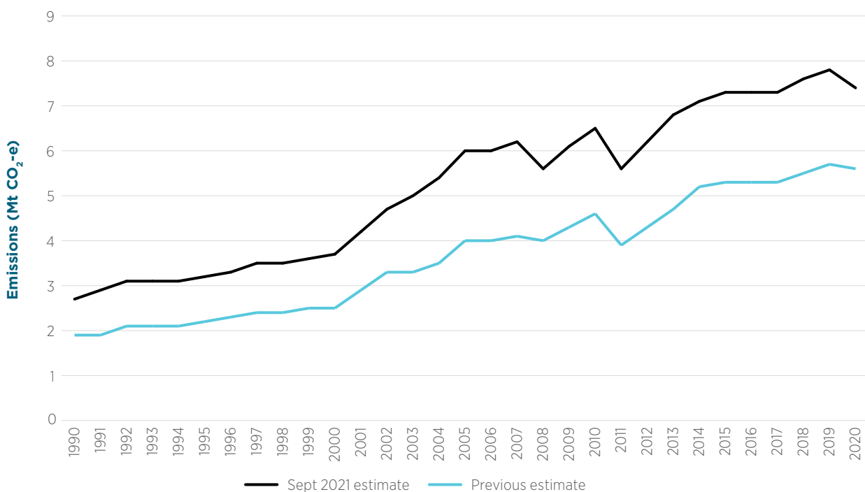
Figure 3.26 Fugitive emissions estimates for QLD surface coal mines
