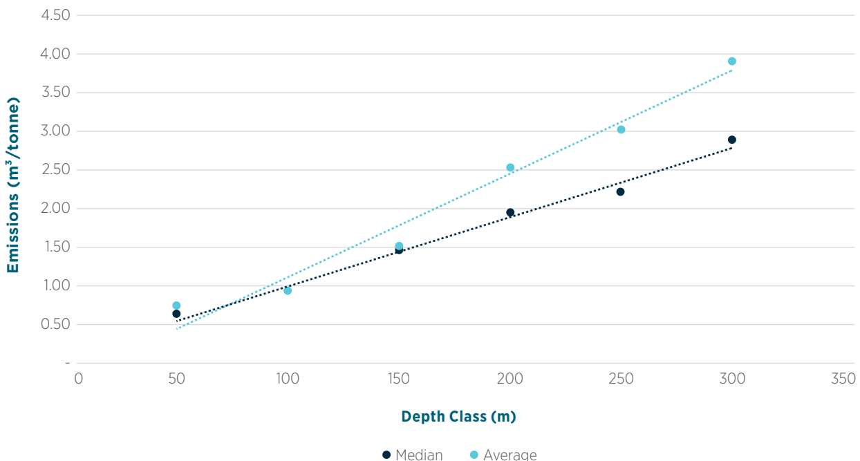
Figure 3.25 Methane content by depth of measurement
