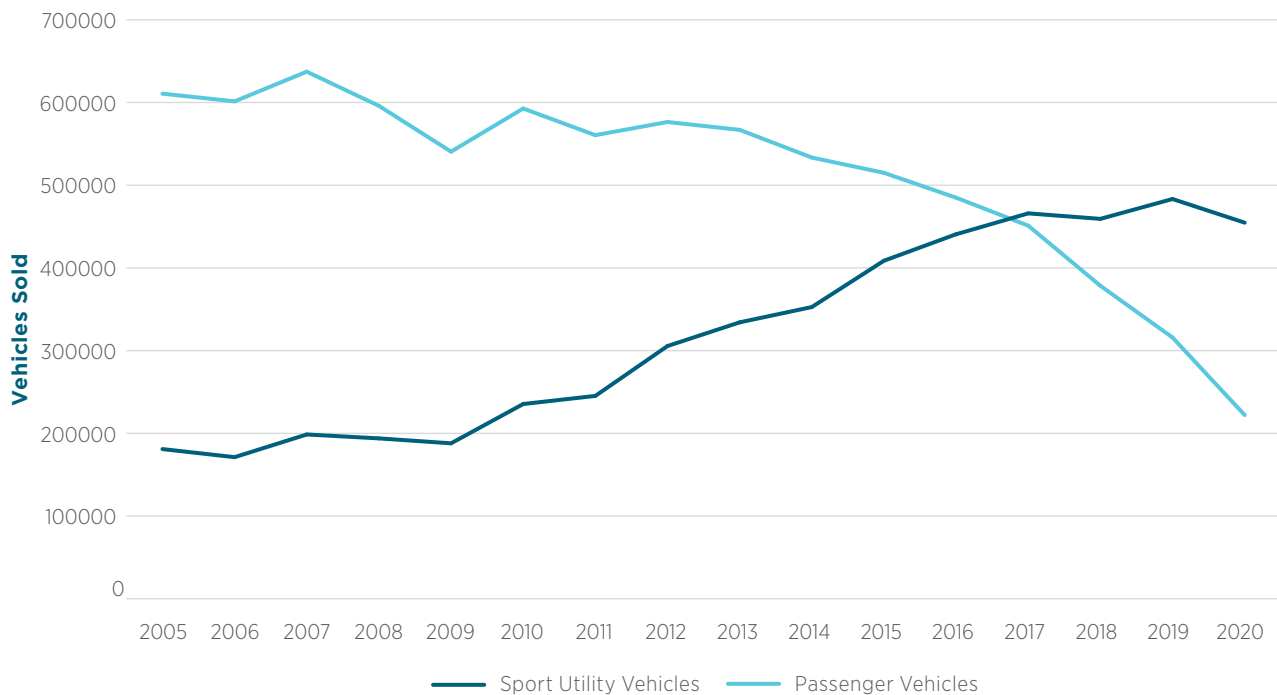
Figure 3.6 SUV and passenger vehicles sales trend in Australia, 2005–2020
