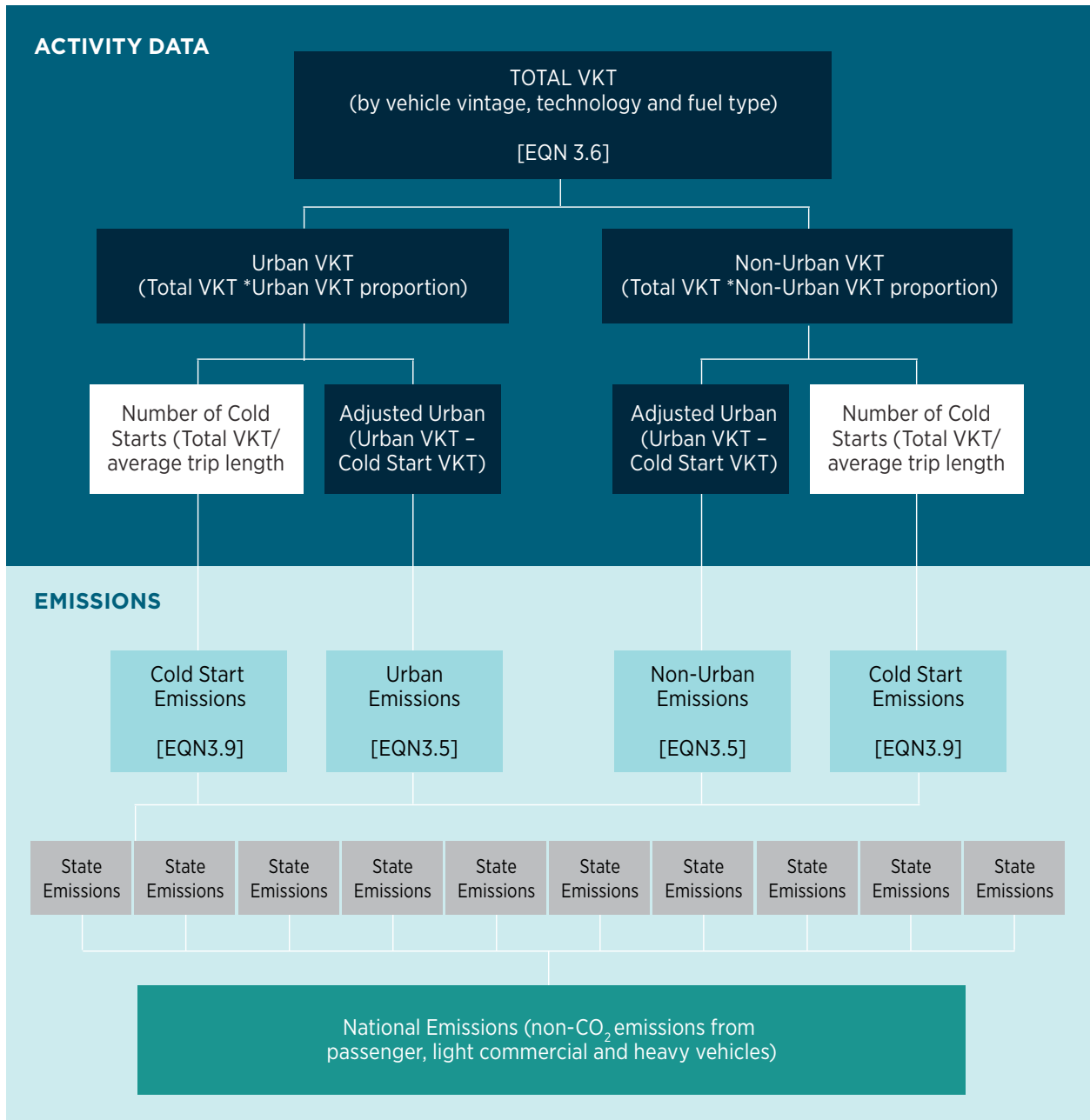
Figure 3.12 Methodology for the estimation of non-CO 2 emissions from passenger and light commercial vehicles
