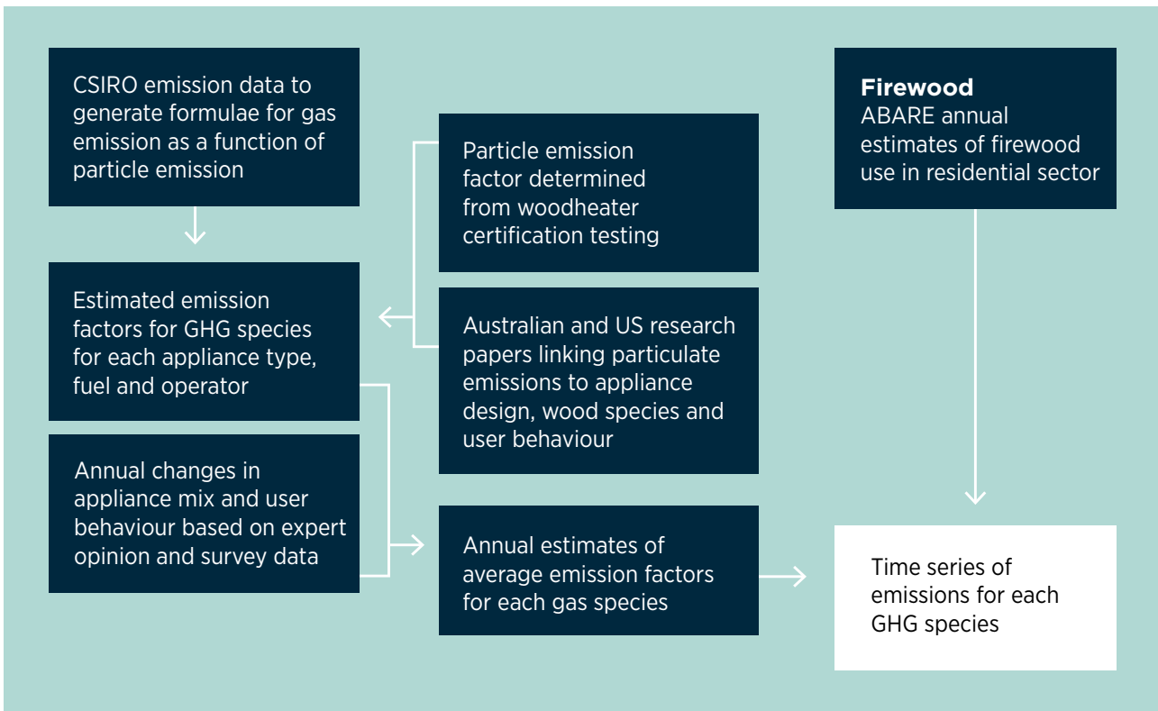
Figure 3.14 Schematic diagram of the methodology process for estimation of emissions from wood heaters
