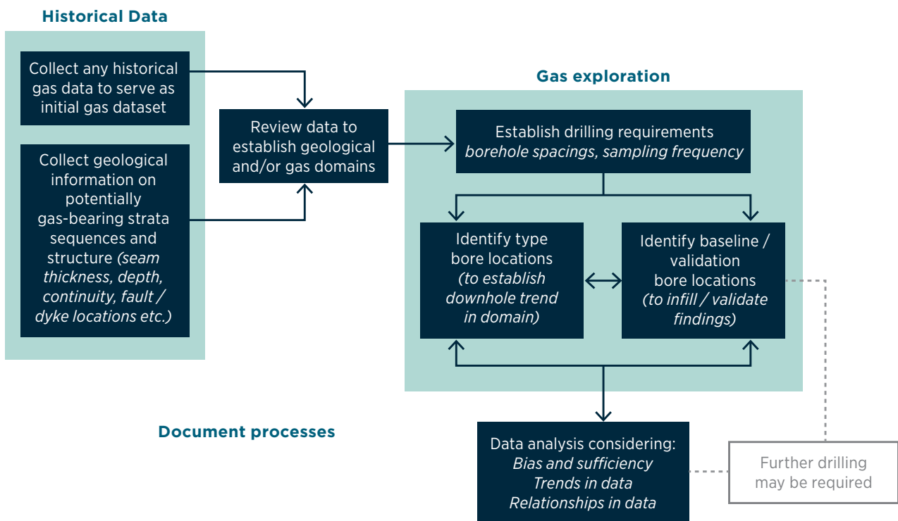
Figure 3.20 Surface mine sample collection process flowchart
