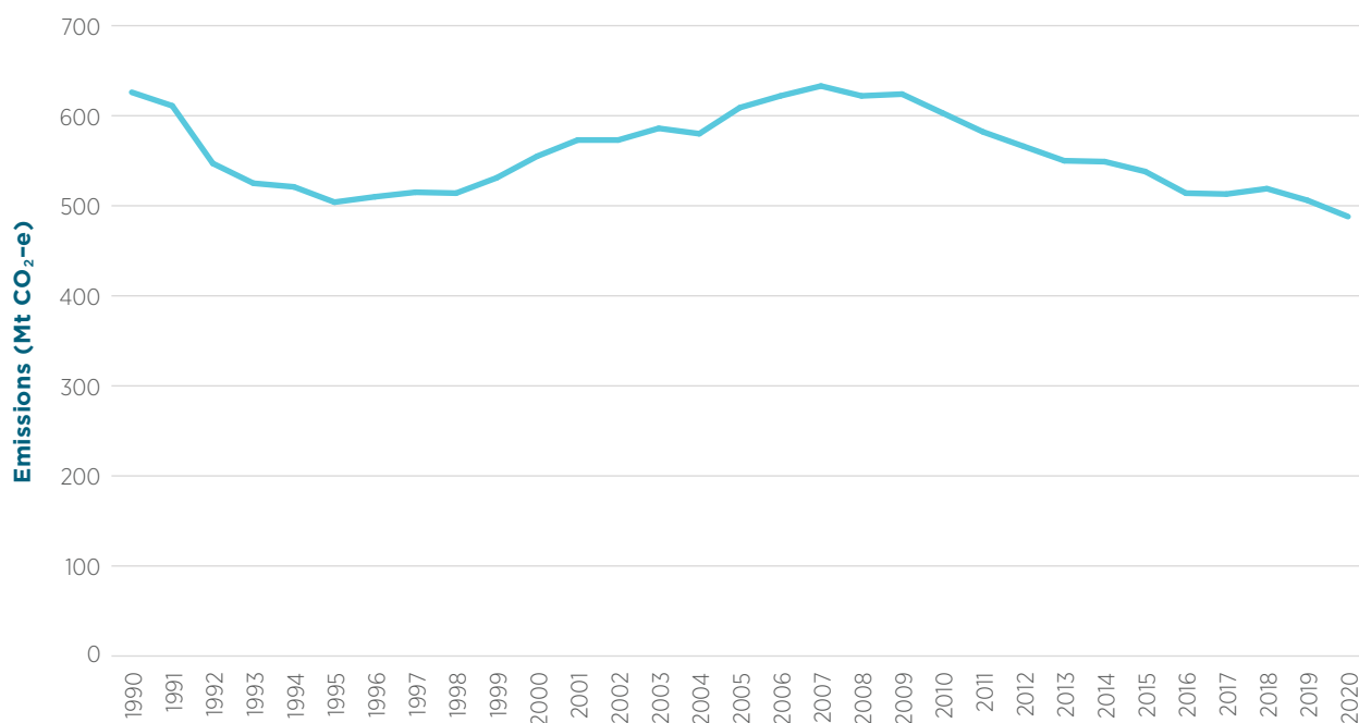
Figure 2.1 National Inventory trend for aggregated greenhouse gas emissions (including LULUCF), Australia, 1990–2020
