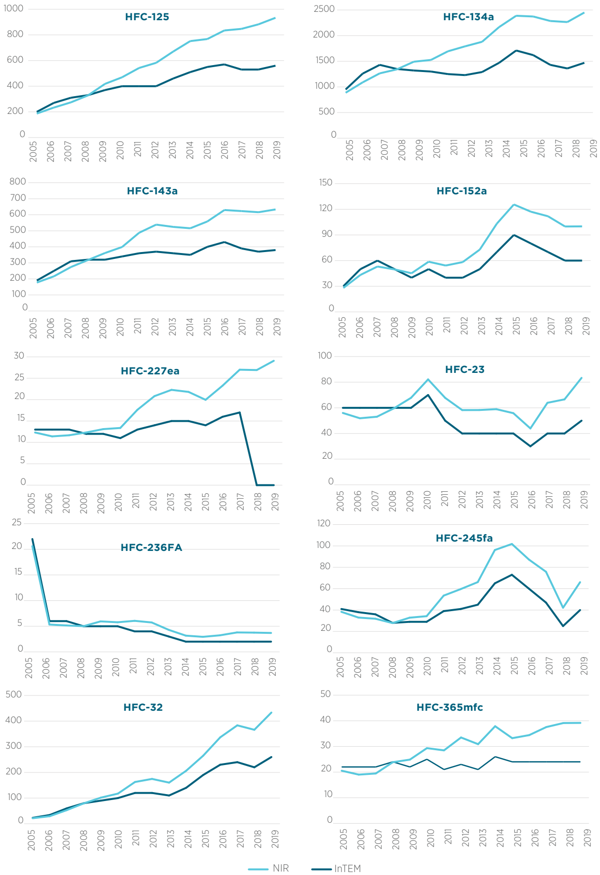
Figure 4.10 Comparison of HFC emissions by species (t)
