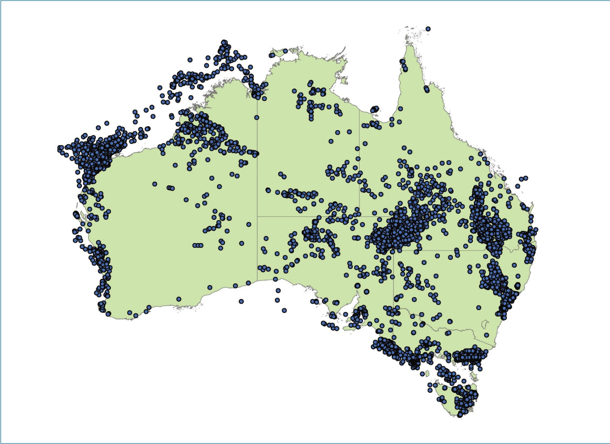
Figure 3.28 Map of abandoned oil and gas wells
