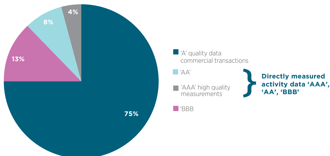
Figure 1.6 Activity data selected by NGER reporters by percentage of data points
