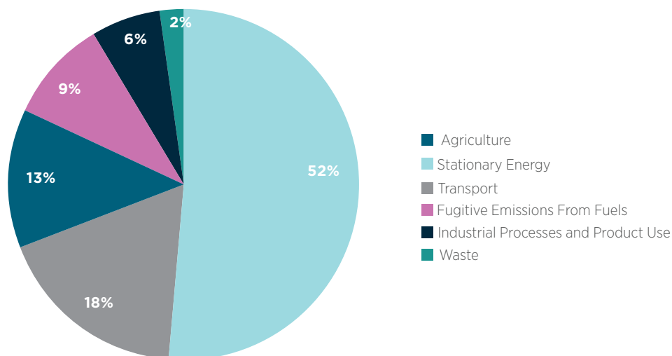
Figure 2.2 Contribution to total net CO 2 -e emissions (excluding LULUCF) by sector, Australia, 2020
