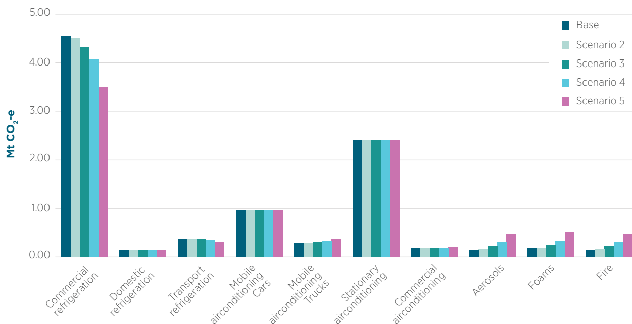
Figure 4.11 Halocarbons: sensitivity testing of allocation assumptions: 2008 (Mt CO 2 -e)
