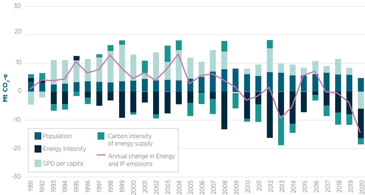
Figure 2.7 Annual change in CO 2 emissions from fuel combustion and IPPU from underlying drivers: Australia 1991–2020 (Mt CO 2 -e)
