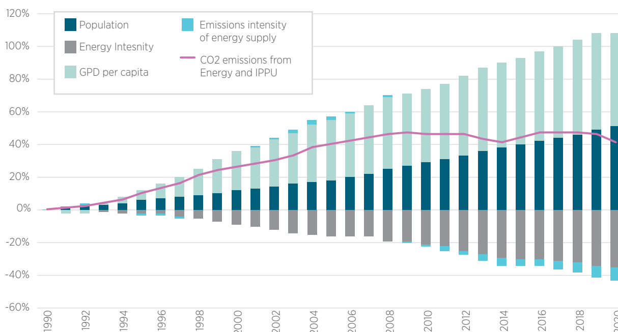
Figure 2.6 Growth in CO 2 emissions from fuel combustion and IPPU and underlying drivers, Australia, 1990–2020
