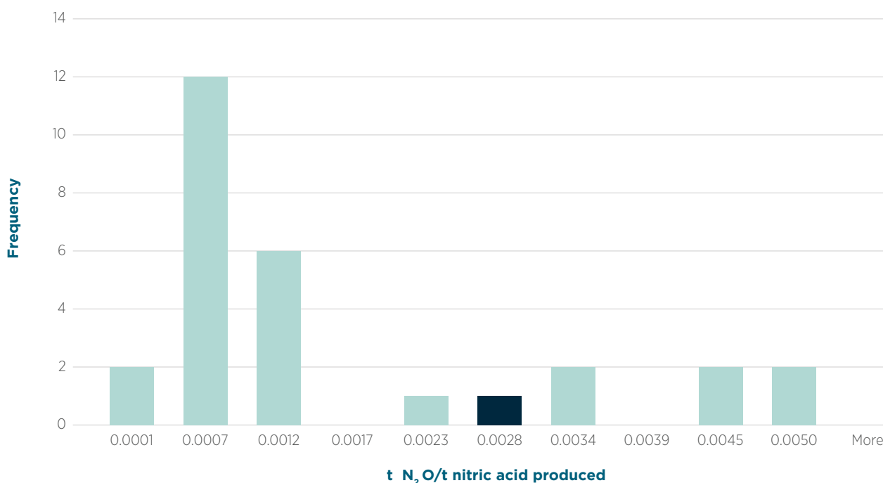
Figure 4.6 Nitric acid implied emission factors for Annex I countries (2019 Inventory) and Australia (2020 Inventory)
