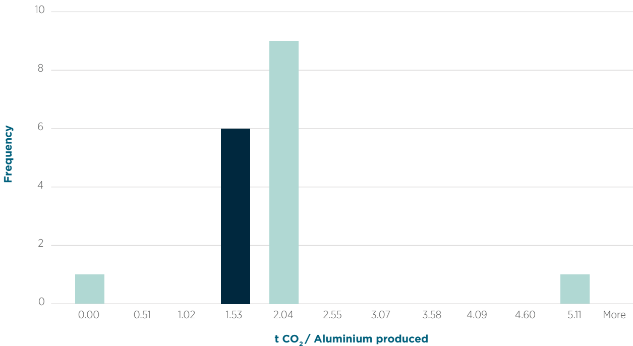
Figure 4.7 Aluminium production implied emission factors for Annex I countries (2019 Inventory) and Australia (2020 Inventory)
