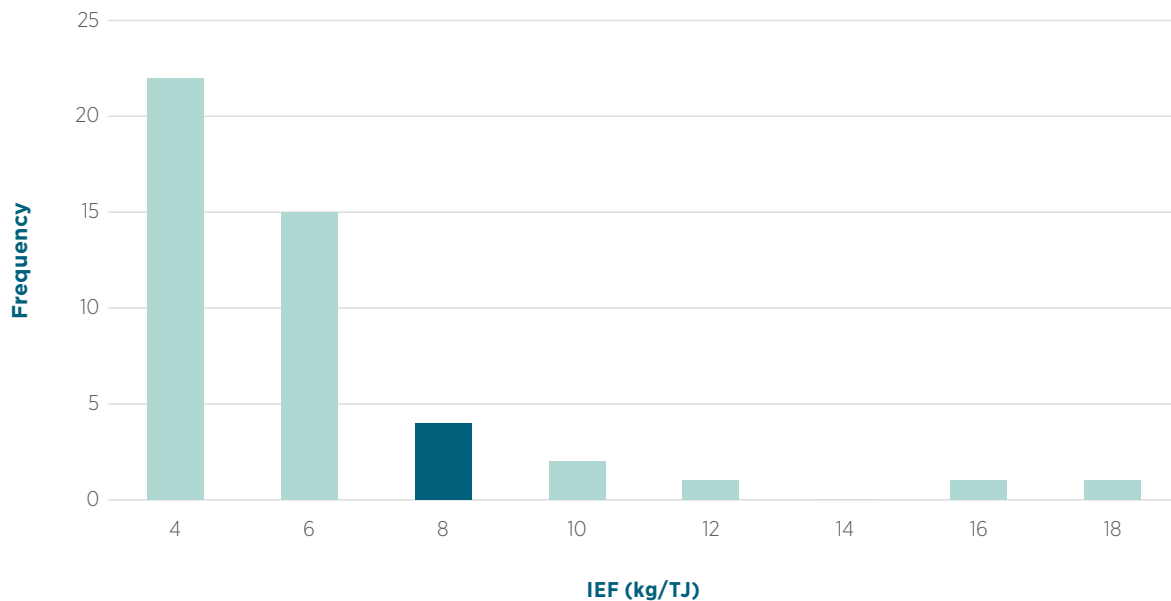
Figure 3.13 2019 methane implied emission factor (IEF) from liquid fuel combustion (kg/TJ) for Annex I countries and 2020 IEF for Australia
