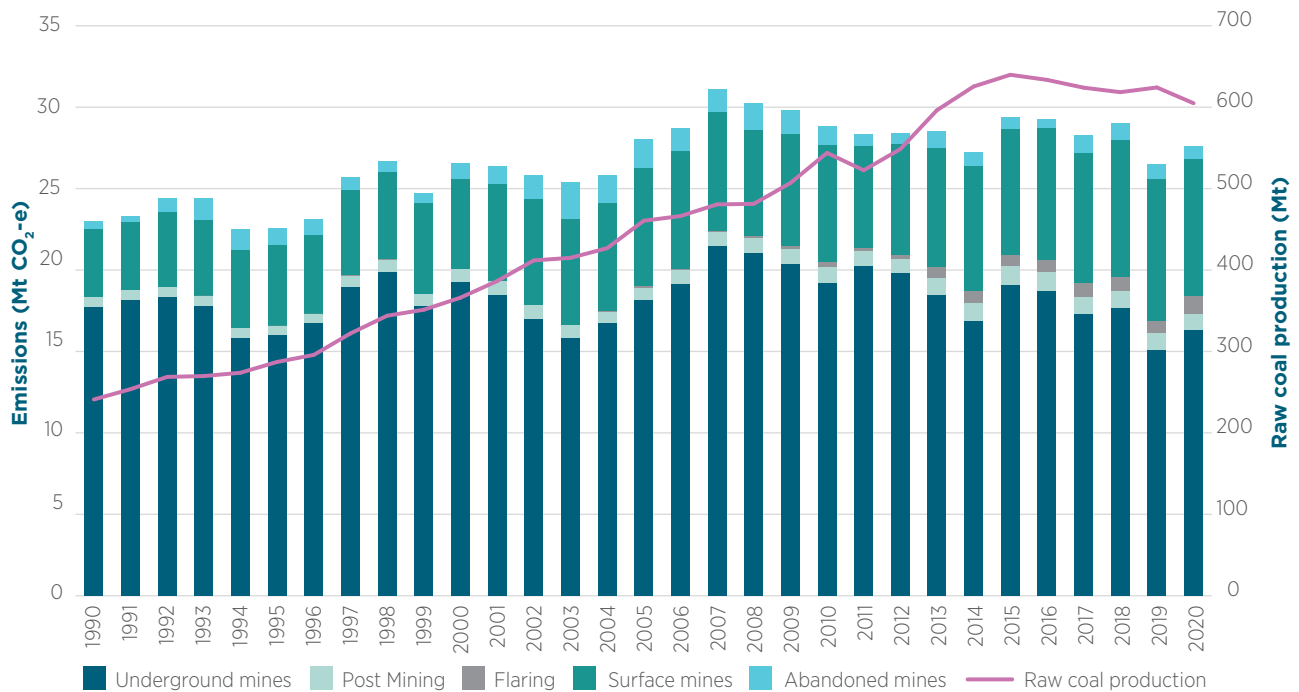
Figure 3.8 Fugitive CO 2 -e emissions from coal mining activities, 1990–2020
