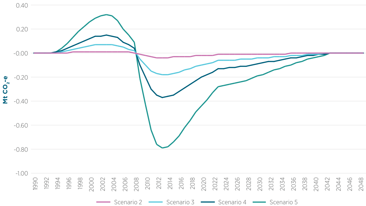
Figure 4.12 Halocarbons: results of sensitivity testing of allocation assumptions: 1990–2050 (Mt CO 2 -e)
