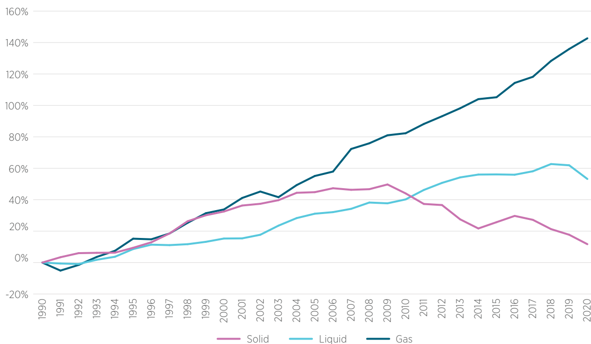
Figure 3.1 Energy sector CO 2 -e emissions by fuel type, percentage change since 1990
