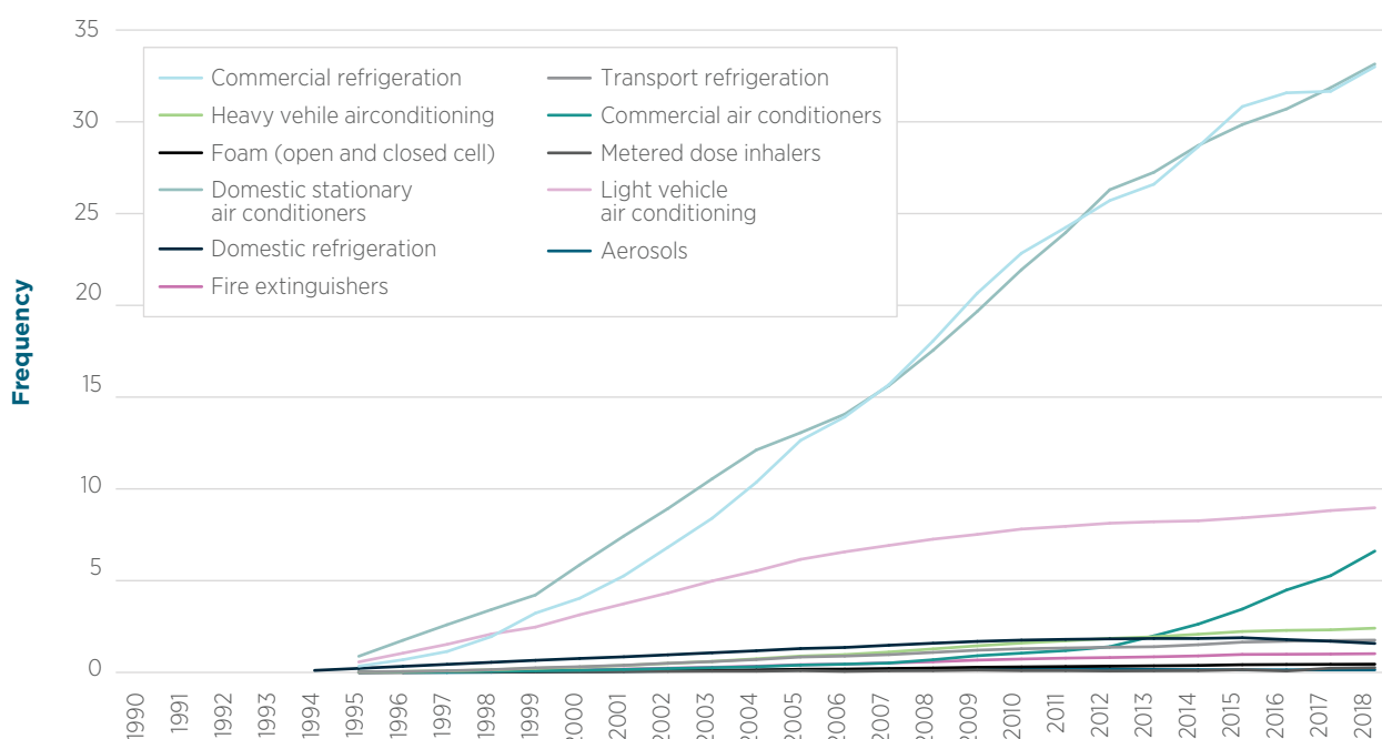
Figure 4.8 Growth in the bank of HF gas in operating equipment (Mt CO 2 -e)
