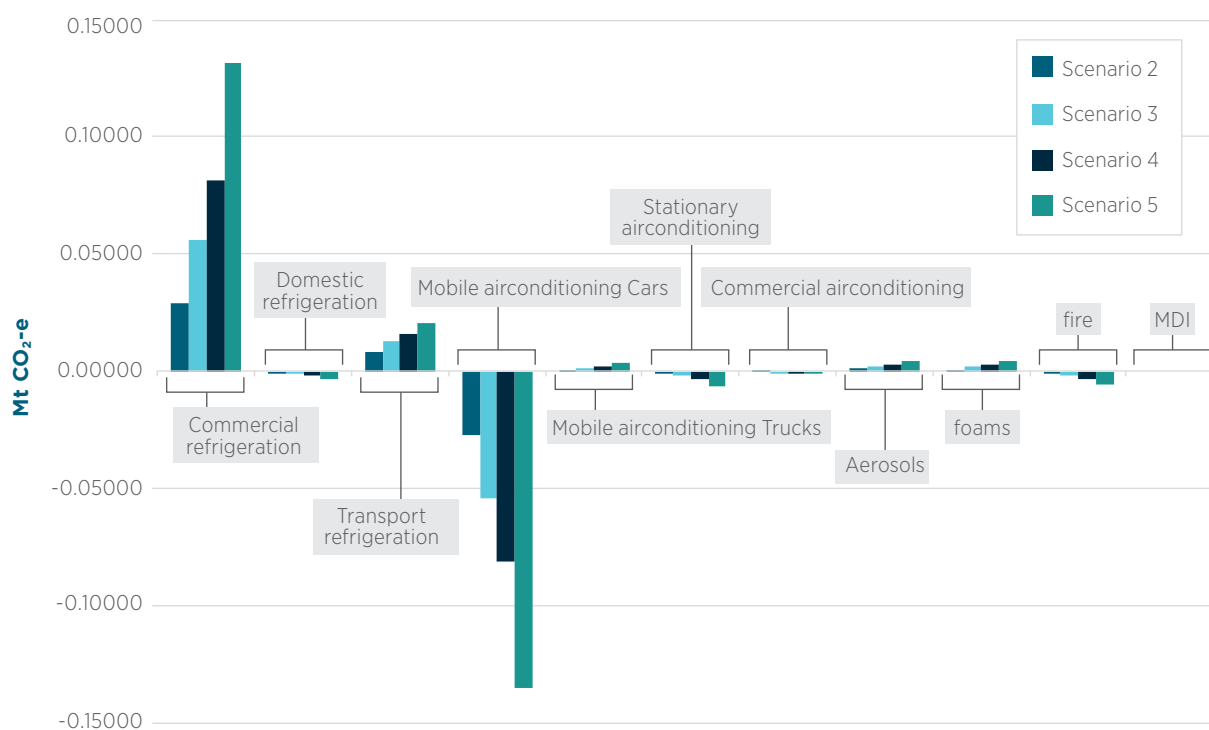
Figure 4.13 Halocarbons: results of sensitivity testing of replenishment assumptions – change in emissions 2008 (Mt CO 2 e)
