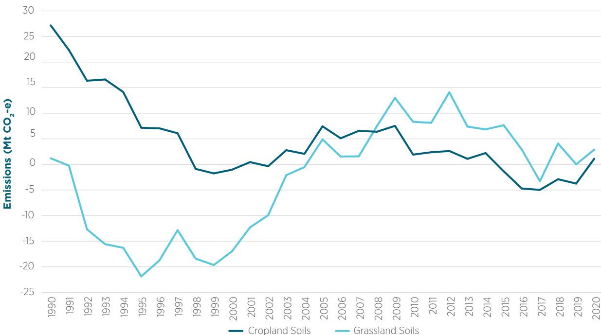
Figure ES.06 Emissions from soils in croplands remaining croplands and grasslands remaining grasslands, 1990–2020 (Mt CO 2 -e)
