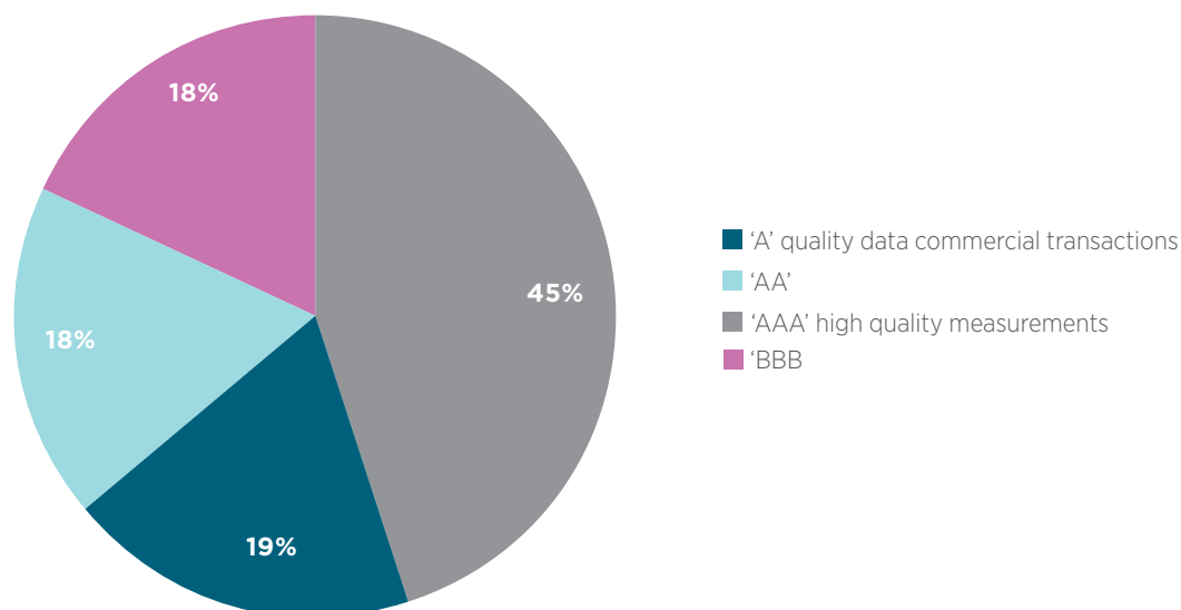
Figure 1.7 Activity data selected by NGER reporters by percentage of emissions
