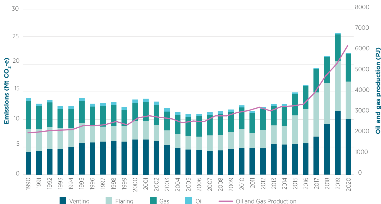
Figure 3.9 Fugitive CO 2 -e emissions from oil and gas production, 1990–2020
