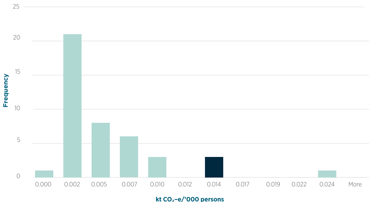
Figure 4.17 N 2 O use implied per capita emission factors for Annex 1 countries and Australia.
