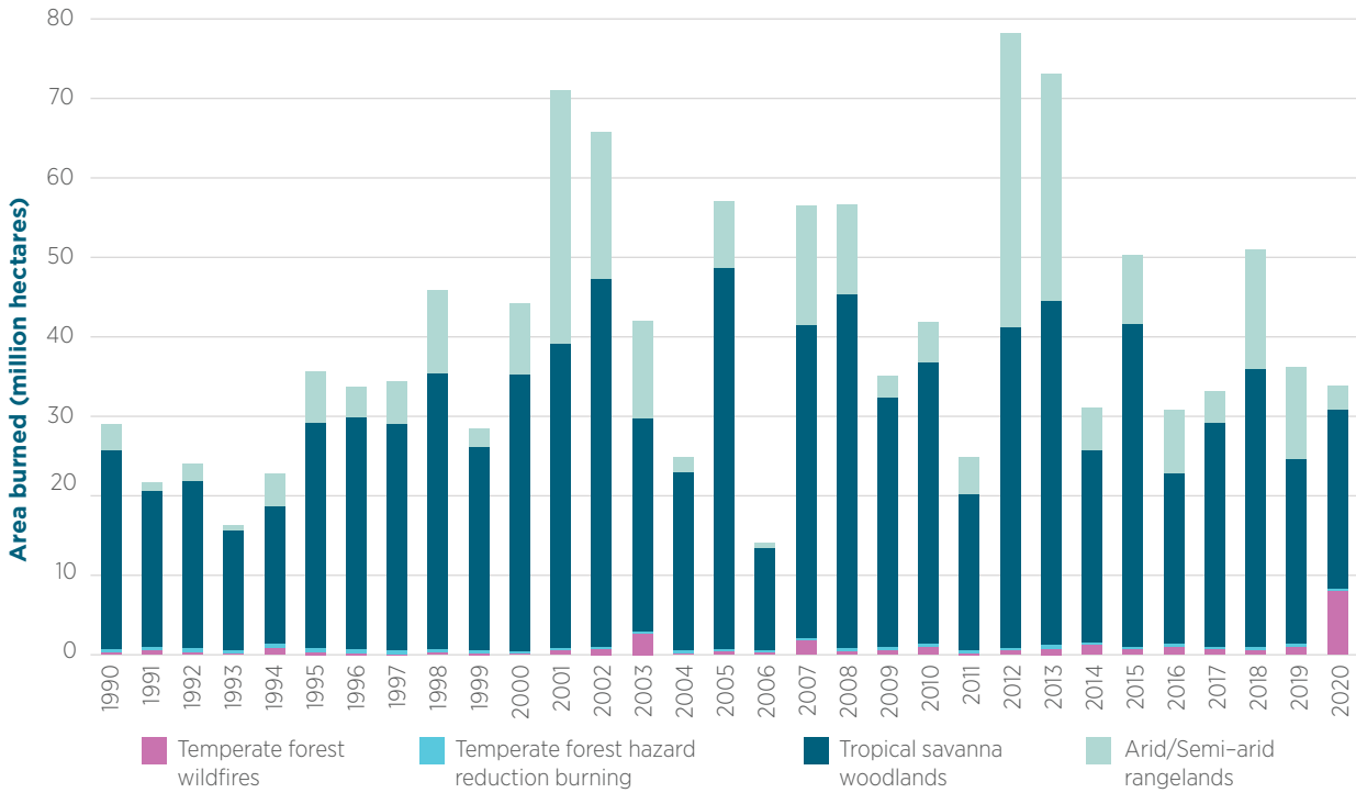
Figure ES.05 Areas of wildfire in Australia, by forest and climate type, 1990–2020 (Mha)
