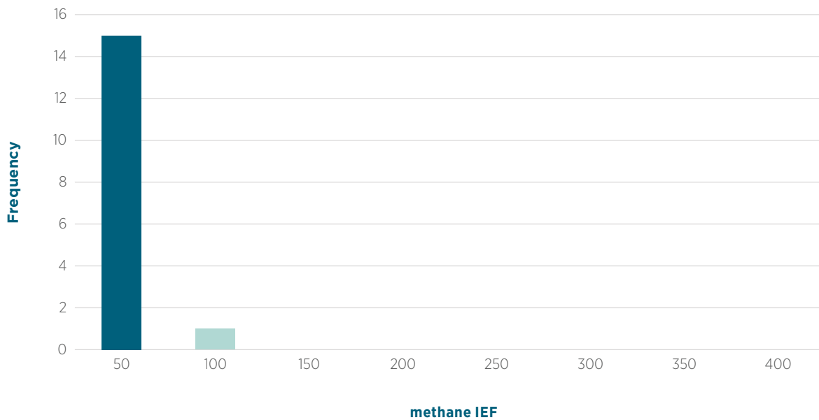
Figure 3.22 Implied emission factor (IEF) for methane from solid fuel underground mine (kg/t) for Annex I countries (2019) and IEF for Australia (2020)
