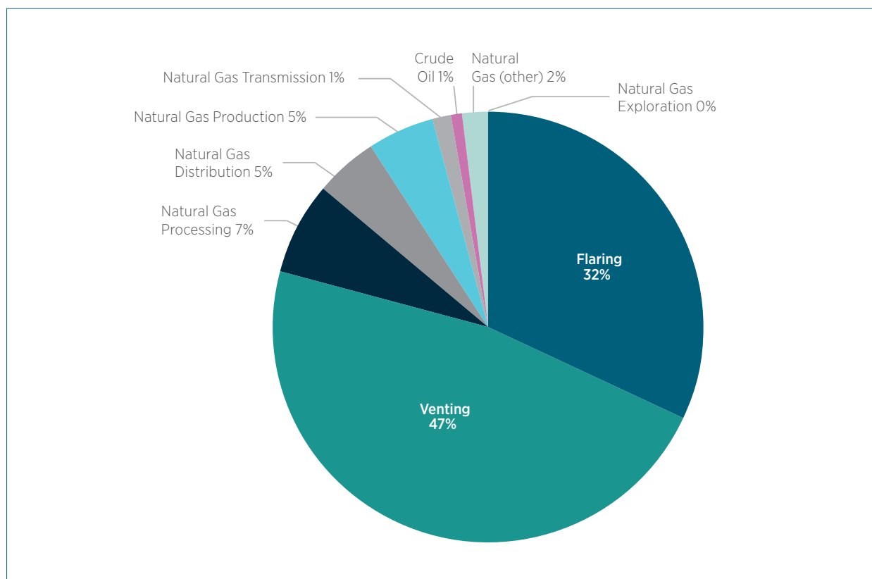
Figure 3.27 Fugitive emissions contribution by oil and natural gas sub-sectors, 2020
