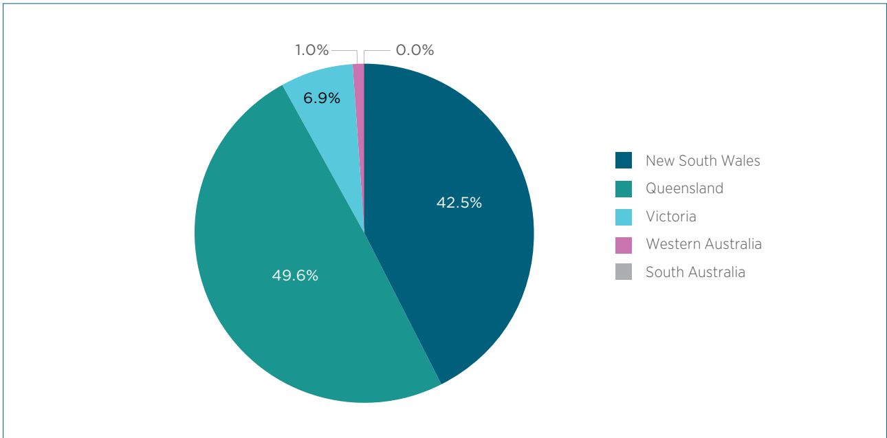
Figure 3.15 Share of coal production from Australian states – 2020
