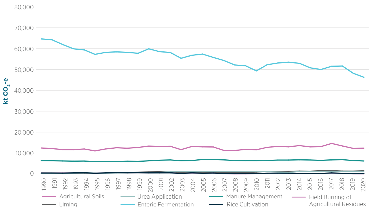
Figure 5.2 CO 2 -e emissions from agriculture, by sub-sector, 1990–2020
