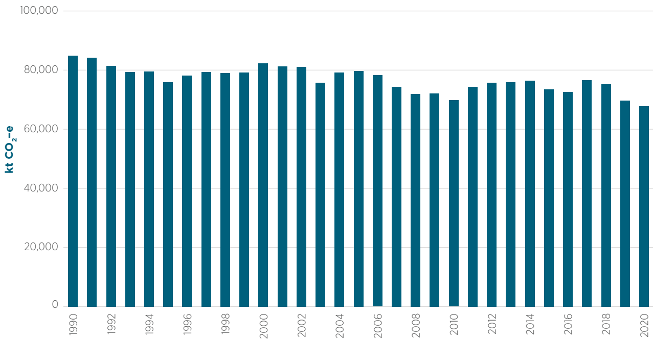
Figure 5.1 CO 2 -e emissions from agriculture, 1990–2020
