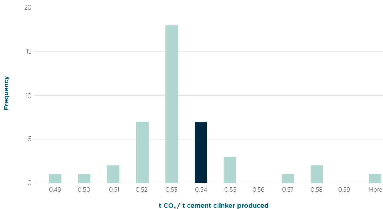
Figure 4.2 Cement production implied emission factors for Annex I countries (2019 Inventory) and Australia (2020 Inventory)
