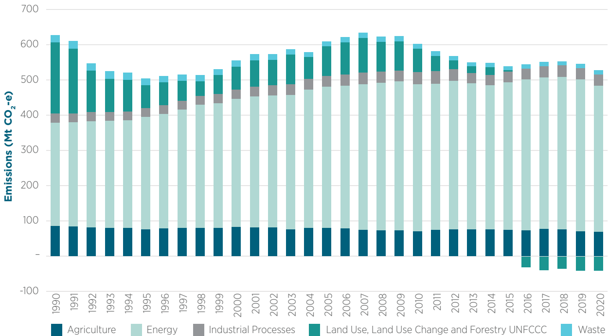
Figure 2.5 Net CO 2 -e emissions by sector, Australia, 1990–2020
