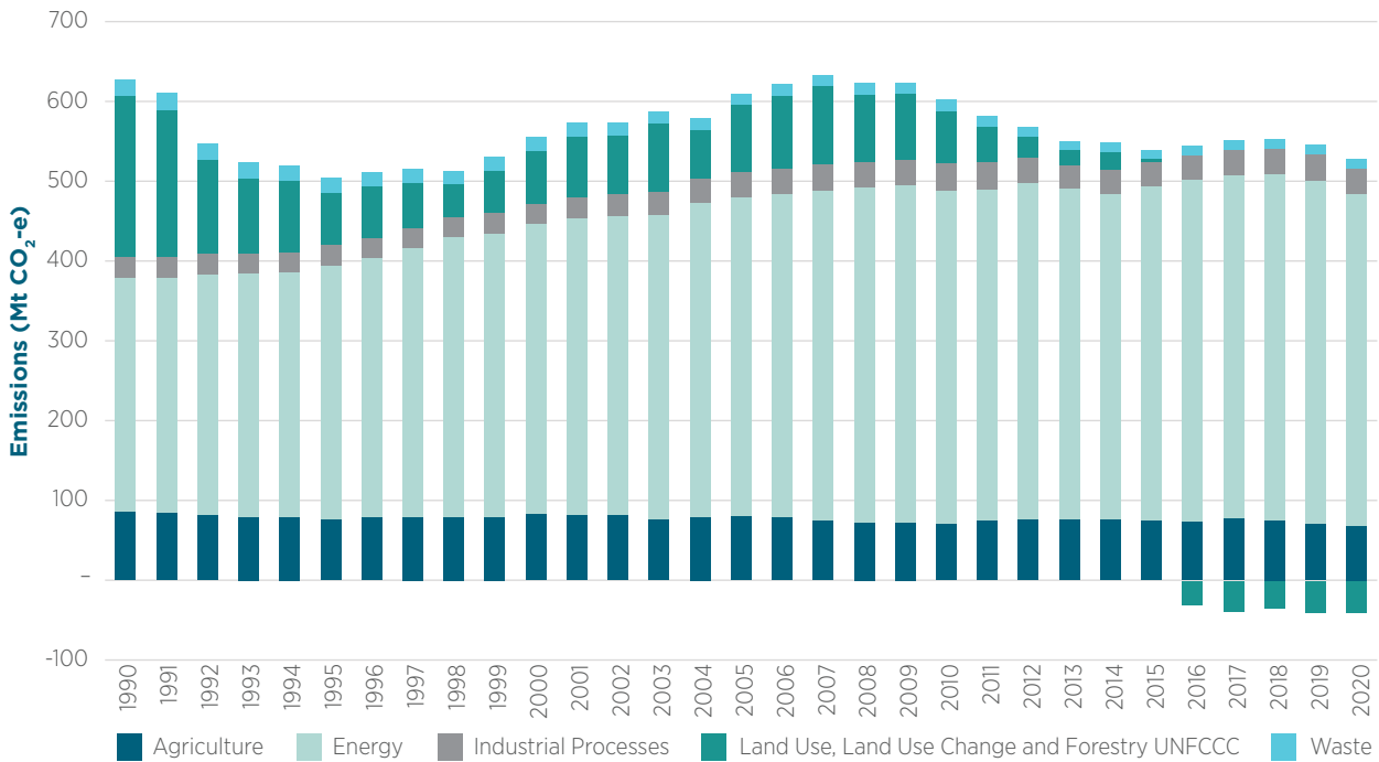
Figure ES.01 Net greenhouse gas emissions under the UNFCCC, by sector, Australia, 1990–2020 (Mt CO 2 -e)
