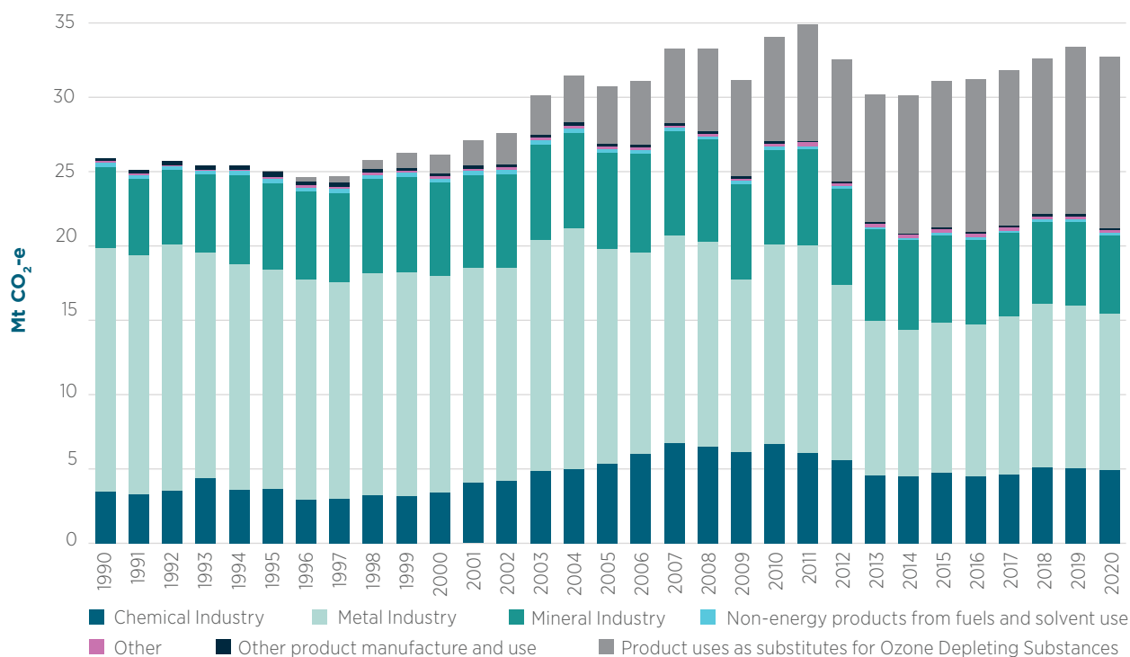
Figure 4.1 Emissions from industrial processes and product use by subsector, 1990–2020
