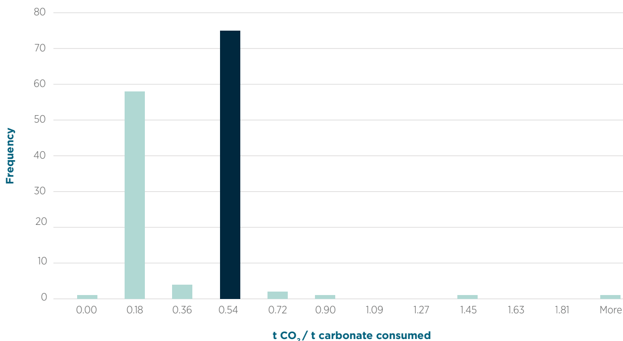
Figure 4.4 Other Process Uses of Carbonates implied emission factors for Annex I countries (2019 Inventory) and Australia (2020 Inventory)
