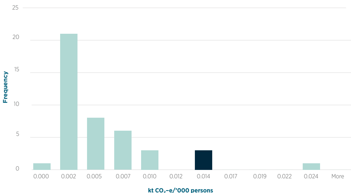
Figure 4.18 Histogram of reported product life emission factors (per cent) by Annex I parties – 2019 (Australia in marked column)
