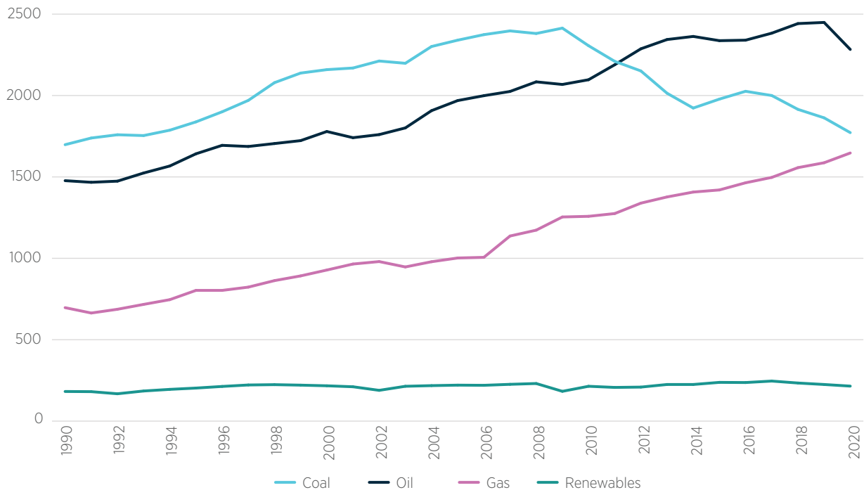
Figure 2.8 Energy consumption by fuel type 1990–2020 (PJ)
