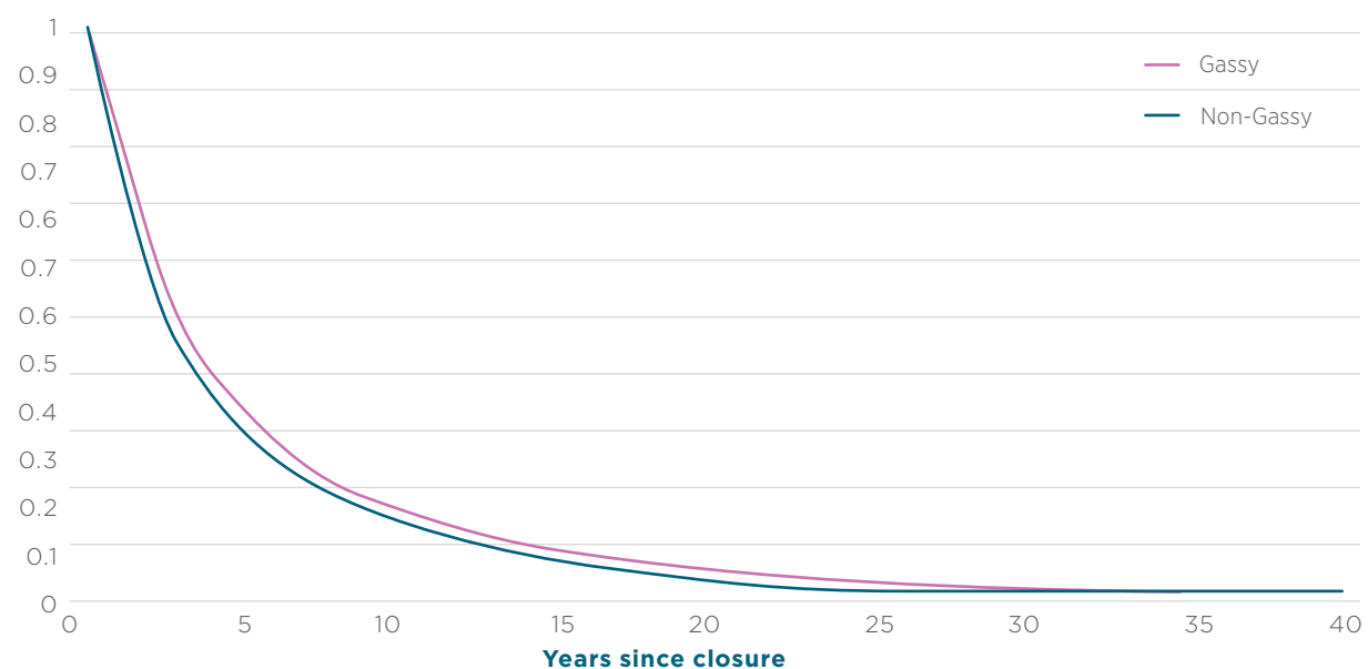
Figure 3.21 Emission decay curves for gassy and non-gassy Australian decommissioned coal mines
