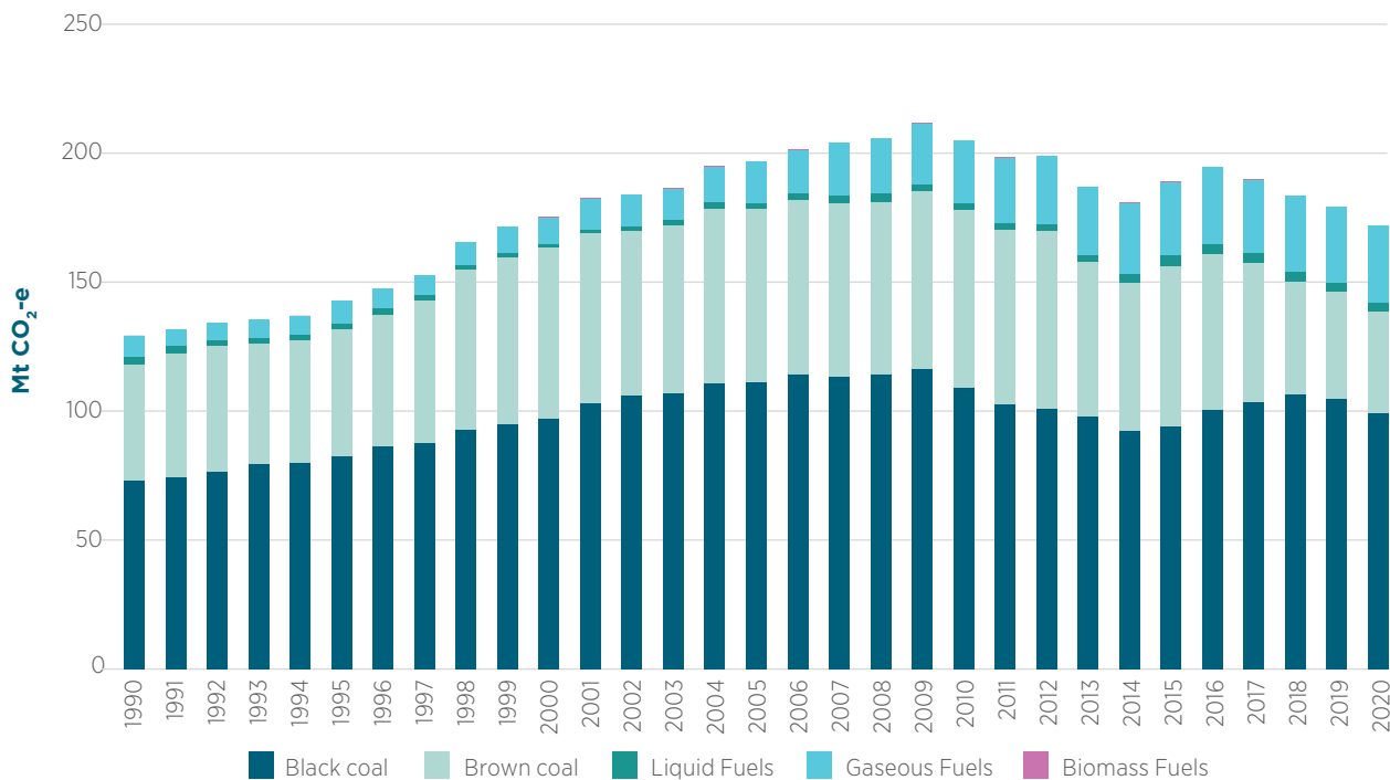
Figure 3.3 CO 2 -e emissions from electricity generation by fossil fuels, 1990–2020
