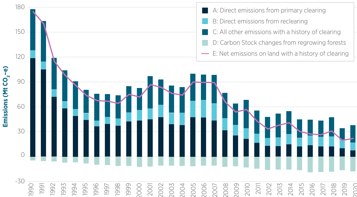
Figure ES.04 Land clearing direct emissions and ongoing emissions from subsequent land use, 1990–2020 (Mt CO 2 -e)
