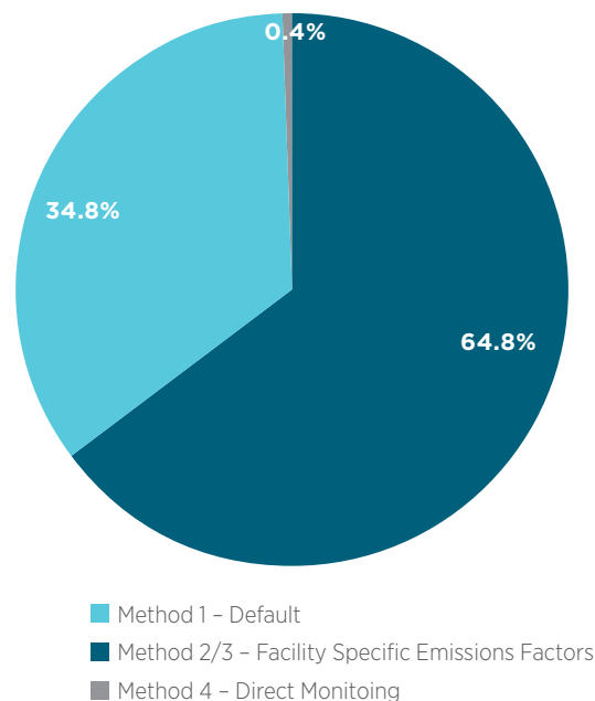
Figure 1.4 2020–21 NGER scheme CO 2 emissions: method selected by NGER reporters
