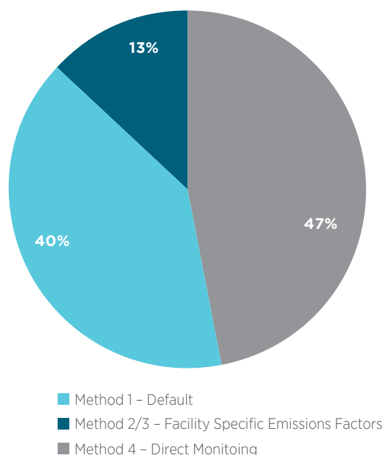
Figure 1.5 2020–21 NGER scheme CH 4 emissions: method selected by NGER reporters
