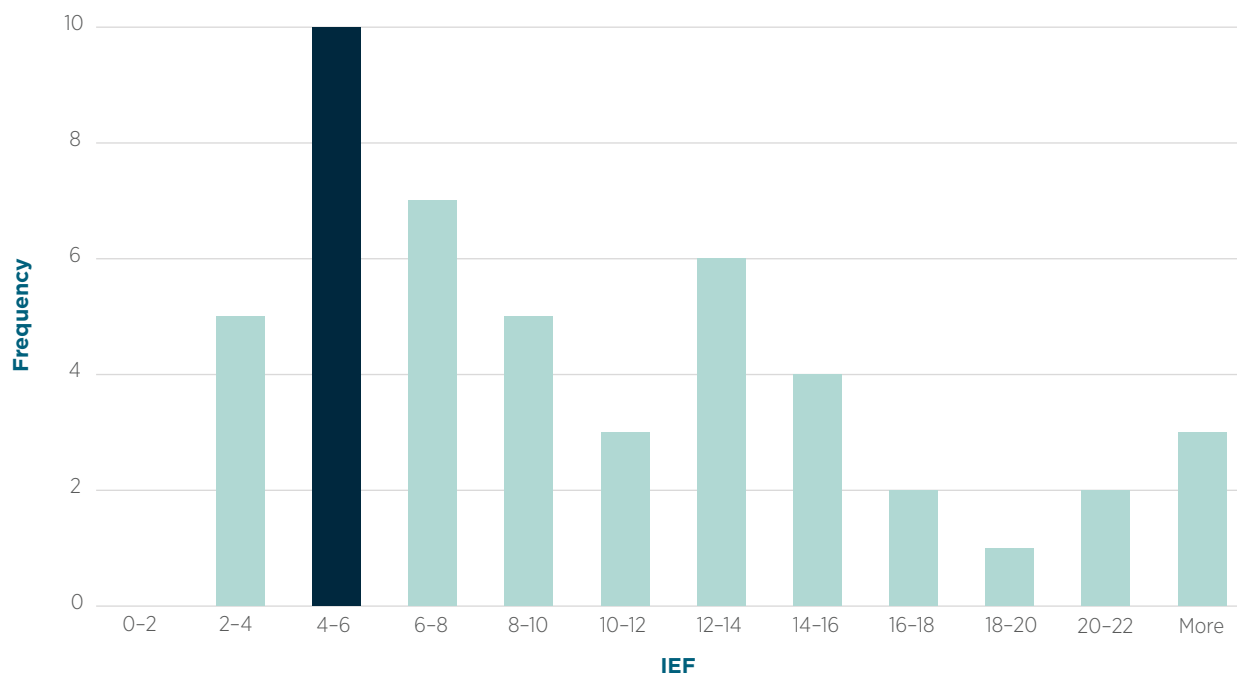
Figure 5.4 Cattle manure management IEF comparisons (kg CH 4 /head/year)
