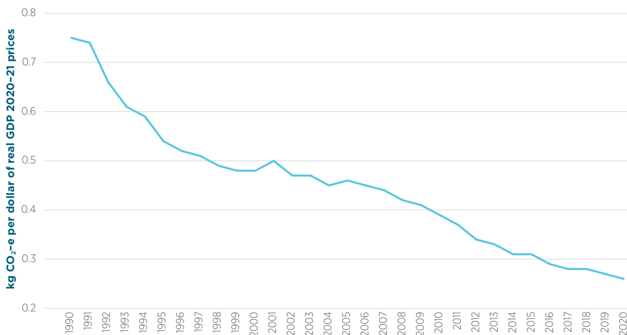
Figure 2.4 Emissions per GDP, Australia (kg CO 2 -e per dollar of real GDP 2020–21 prices)
