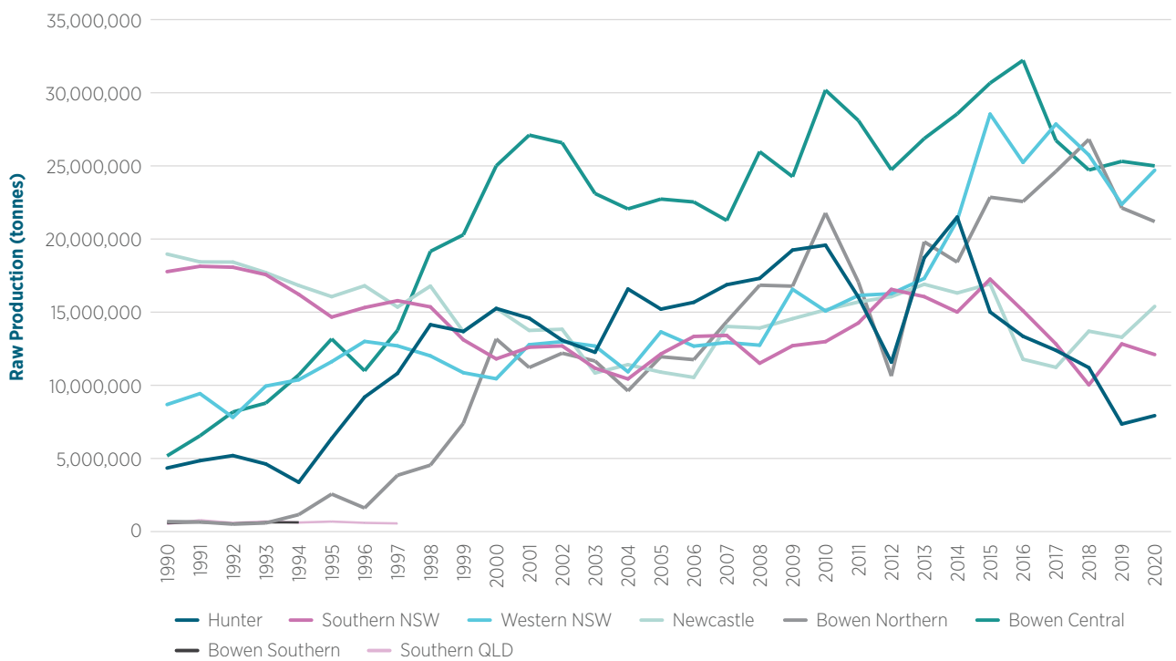
Figure 3.16 Underground black coal production by coal field
